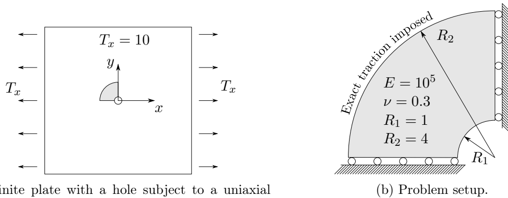
Figure 14: Schematics of infinite plate with a hole.
