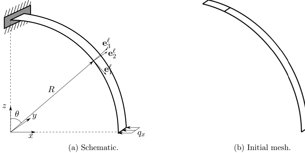
Figure 20: Cylindrical shell subject to transverse loading in the radial direction. \{e_i^l\}_{i=1}^3 is a local Cartesian coordinate basis used for calculating resultant forces [1].
