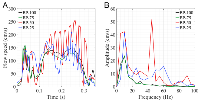
Fig. 3. Flow speed results for each valve thickness case. (A) The speed is evaluated for each valve at the point indicated in Fig. 1B. (B) Frequency domain from the discrete Fourier transform operations for t = 0.1 to 0.3 s of the flow speed.
