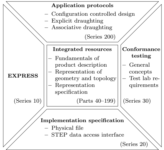
Fig. 32: Structure of STEP (re-execution of the original diagram [177]).
