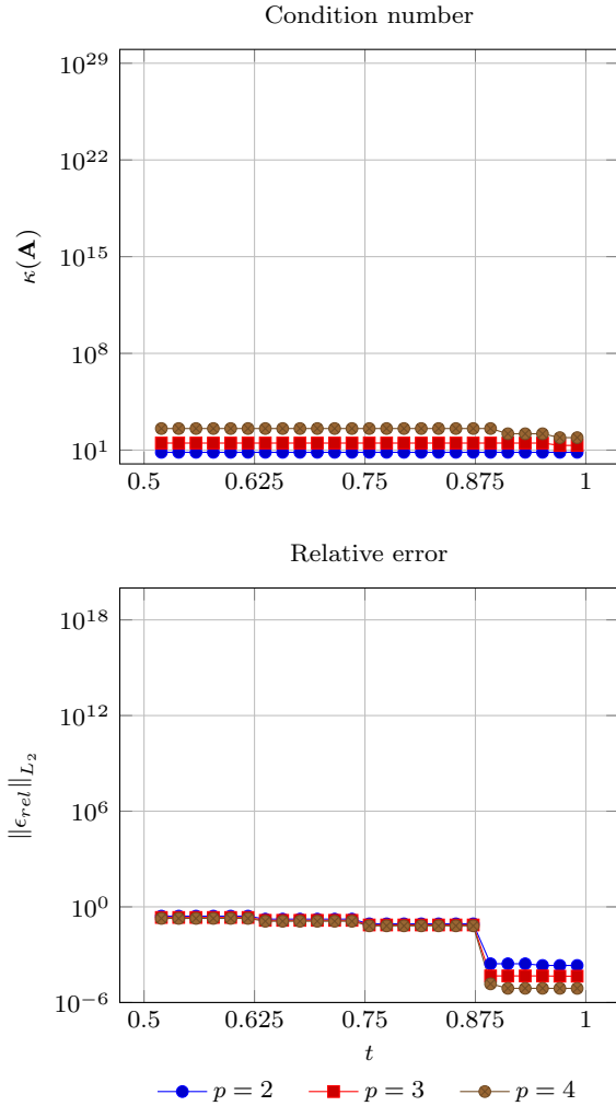
Fig. 67: Spline interpolation problem with extended B-splines for several orders p . The condition number \kappa(\mathbf{A}) and the relative interpolation error \|\epsilon_{rel}\|_{L_2} are related to the trimming parameter t . The labels of the horizontal axis indicate knots of the trimmed basis.
