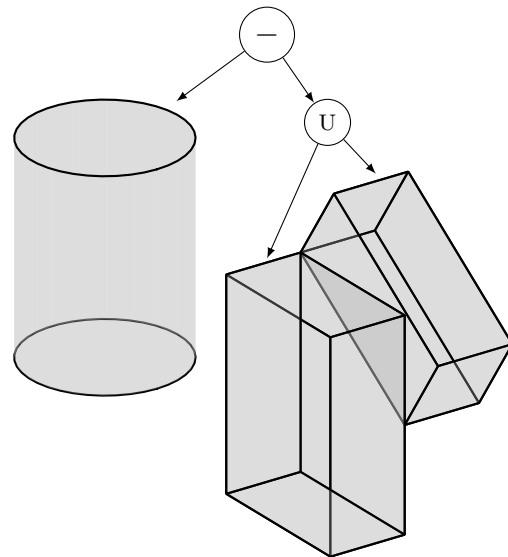
Fig. 18: Representation of the object shown in Figure 12(a) by means of a CSG tree: the object is specified by a composition of simple solids using Boolean operations, i.e. union (U) and difference (-).
