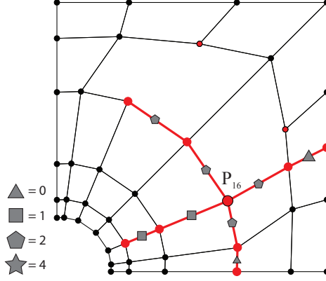
Figure 3: Constructing the local knot interval vectors corresponding to T-mesh vertex \mathbf{P}_{16} .
