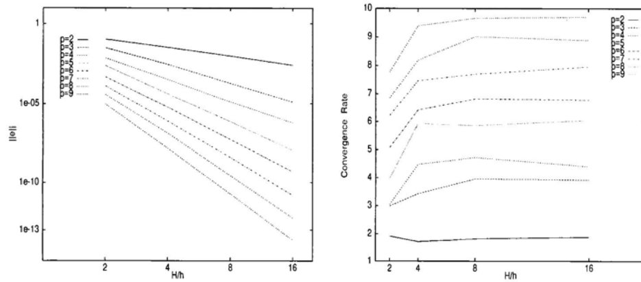
FIG. 12. Distorted domain: -\Delta \psi = S , S = -\Delta(\exp(-(x^2 + y^2))) .
