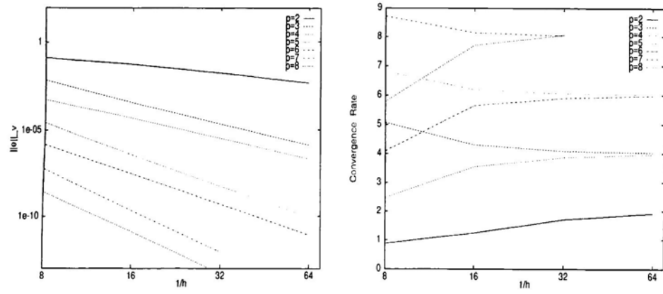
FIG. 7. V -norm of the error and convergence rate with uniform meshes: -\partial^2 u / \partial x^2 = S , S = (4\pi)^2 \sin(4\pi x) .
