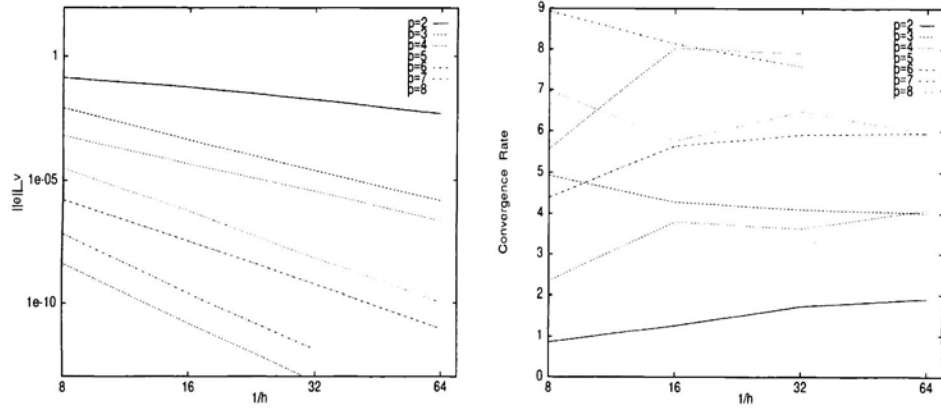
FIG. 8. V -norm of the error and convergence rate with nonuniform meshes: -\partial^2 u / \partial x^2 = S , S = (4\pi)^2 \sin(4\pi x) , \delta h = \pm 20\% .
