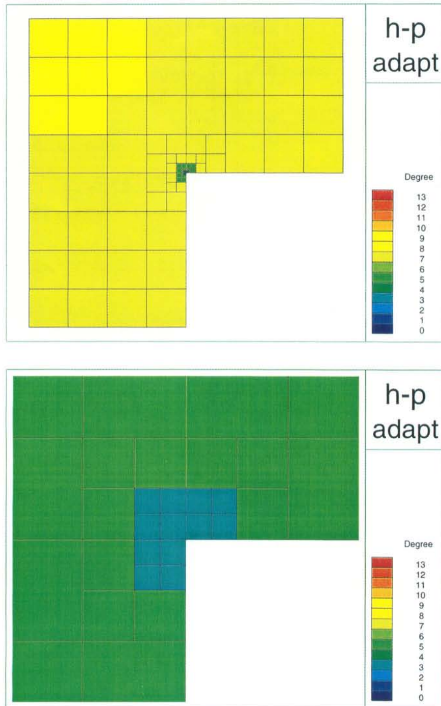
FIG. 13. L -shaped domain. Top: Mesh and polynomial basis after h-p adaptation, Bottom: close-up view \times 20 at the corner.
