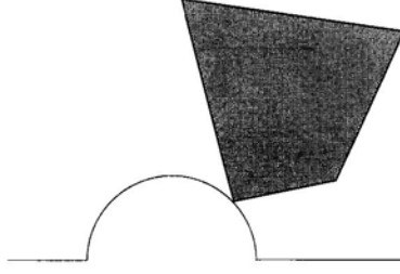
FIG. 3. Subdomain for successive global refinements.
