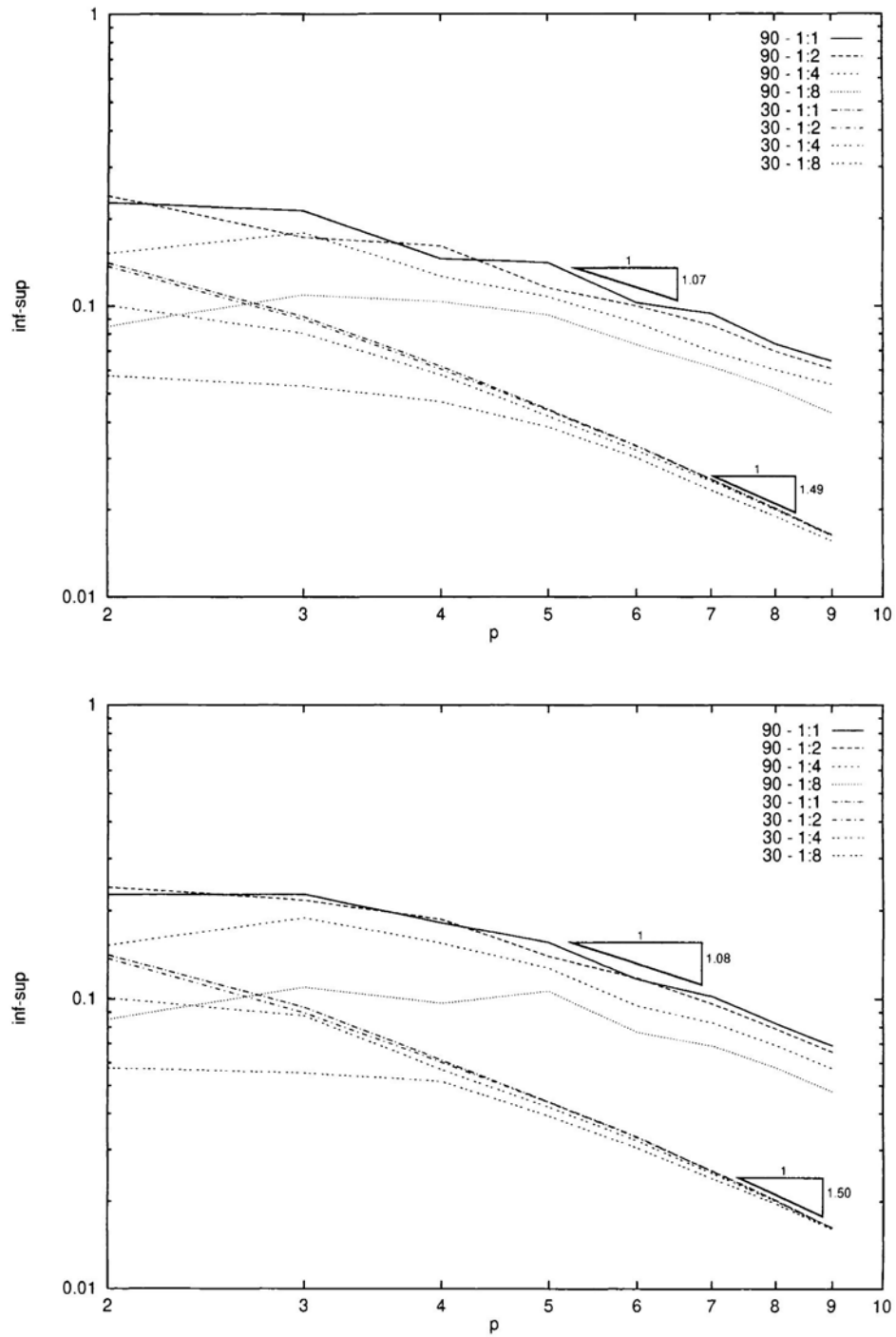
FIG. 6. Inf-sup values for a mesh with 64 elements. Top: uniform p . Bottom: random distribution of p .
