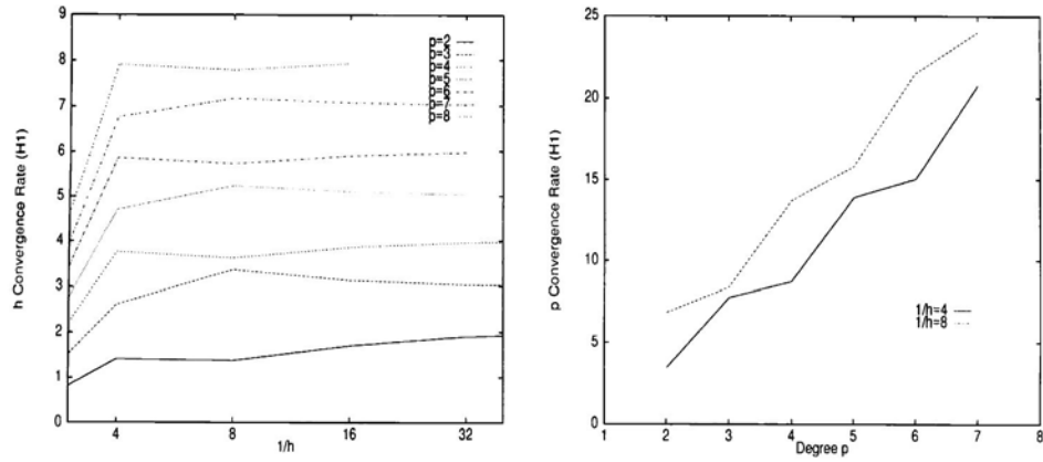
FIG. 11. h and p convergence rates in the H^1 seminorm: -\partial^2 u / \partial x^2 = S , S = (3\pi)^2 \sin(3\pi x) .
