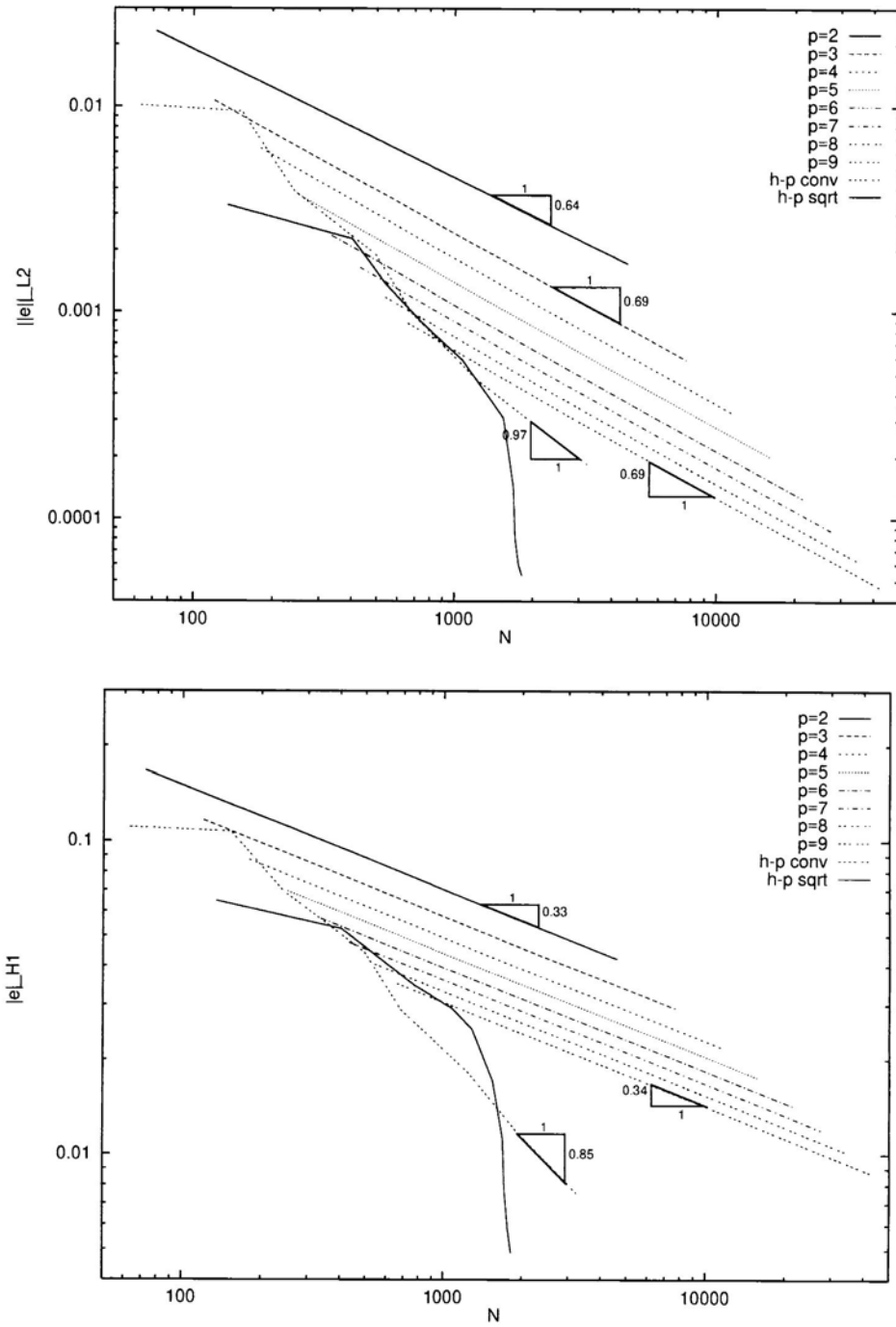
FIG. 18. L -Shape domain: Convergence rates using global and adaptive refinements. Top: L^2 norm. Bottom: H^1 seminorm.
