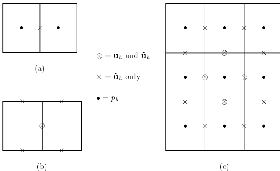
Fig. 1. Nodal points for the standard basis functions ( d = 2 ). (a) Stencil for the dependence of \tilde{\mathbf{u}}_h on p_h . (b) Stencil for the dependence of \mathbf{u}_h on \tilde{\mathbf{u}}_h . (c) Stencil for the pressure p_h .
